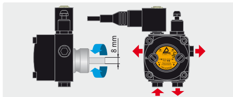
Pump VU. Single line intake or double line intake. Cable 700 mm. Pressure adjustable 6 - 18 bar
