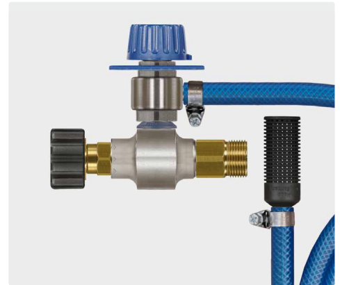
M22 F : M22 M. Injector with metering valve ST-161, suction hose 2,000 mm and suction filter ST-31. Max. 350 bar / 90 °C
