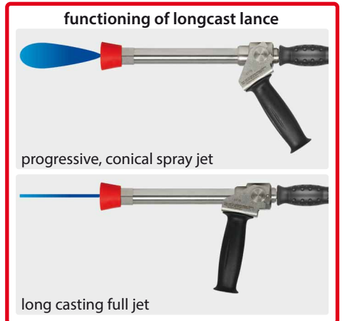
1/2" F. Stainless steel. Longcast lance 350 mm with insulation ST-29 Cool & Compact 330 mm, gun easyfarm365+ , grip aside and nozzle protector made out of plastic without nozzle. Max. 250 bar / 60 l/min / 100 °C
