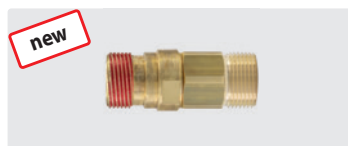
TR 22 M : M22 x 1,5 M. Alternative to adapter 1. Brass. Max. 400 bar.
