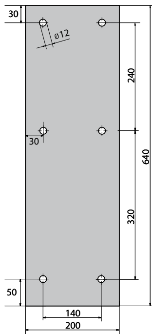
(e) counterplate (opt.) 109 790 419 3
