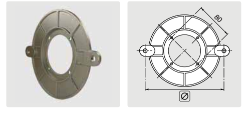
Flange for burner motors
