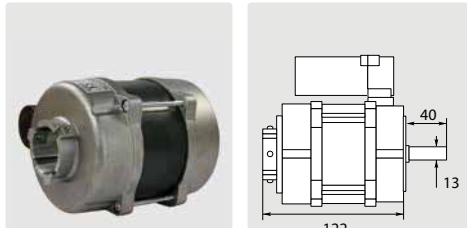
Motor with pump shaft 32 mm
