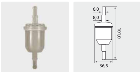
Fuel filter
