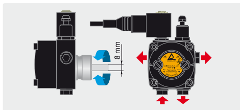
Pump VU. Single line intake or double line intake. Cable 700 mm. Pressure adjustable 6 - 18 bar
