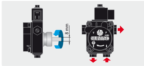
Pump VM. Single line intake or double line intake. Pressure adjustable 7 - 14 bar
