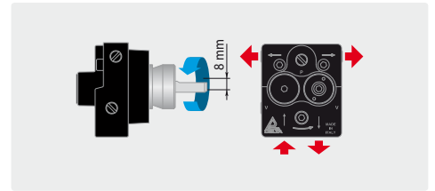
Pump A. Single line intake or double line intake. Pressure adjustable 6 - 20 bar
