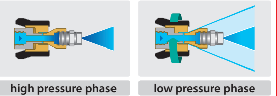
Functional principle of a adjustable nozzle
