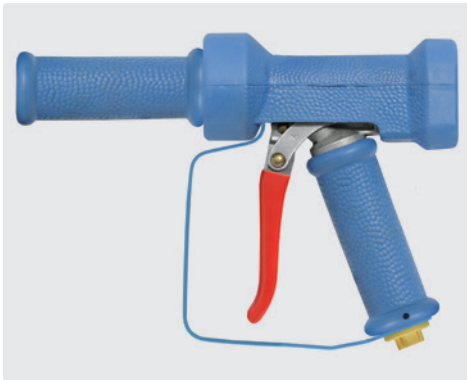
Spray gun with adjustable spray angle. Trigger guard. Max. 24 bar / 100 l/min / 95 °C
