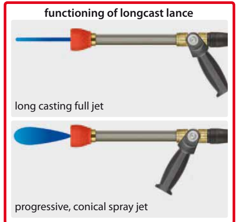
1/2" F. Longcast lance 500 mm with vented handle ST-9.1 260 mm, gun easyfarm365+, grip aside and nozzle protector made out of plastic without nozzle. Max. 180 bar / 60 l/min
