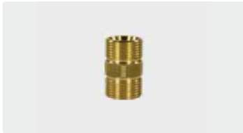
M22 M. Standard. Brass. Max. 400 bar
